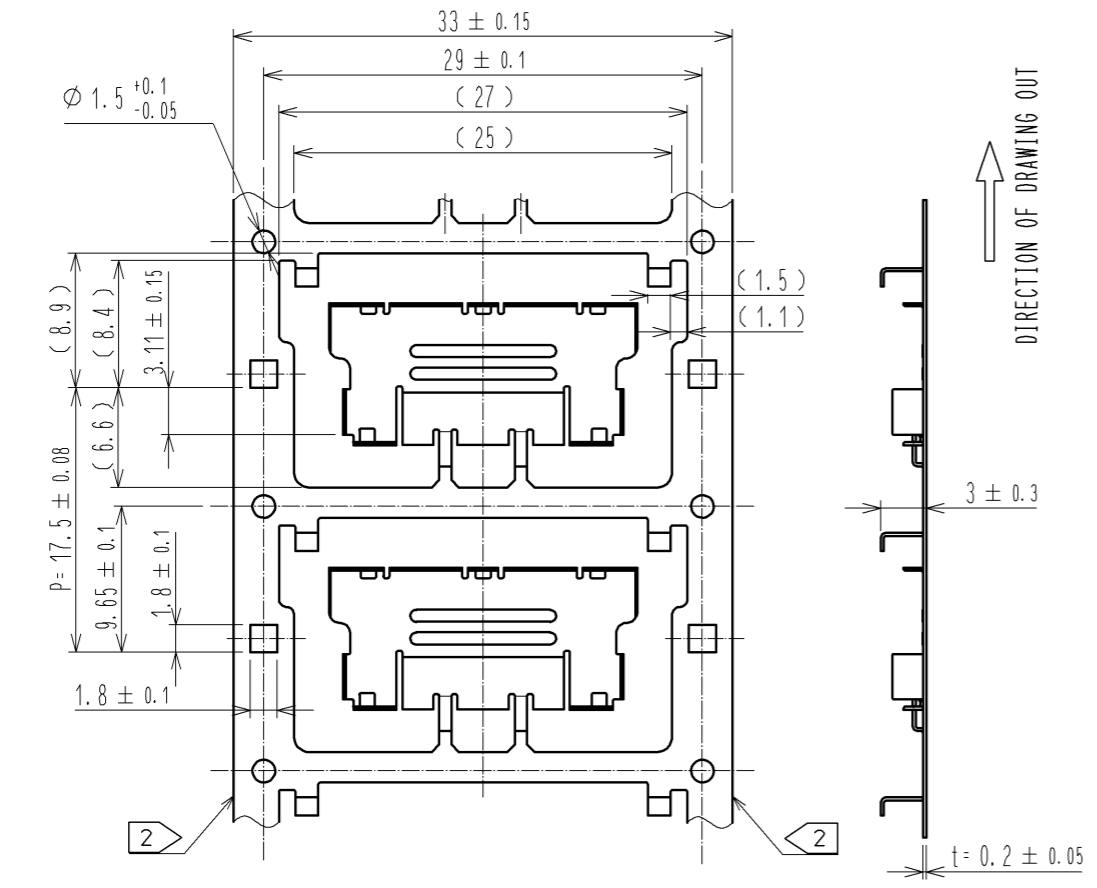
DETAILED FIGURE OF CARRIER (2 : 1)
